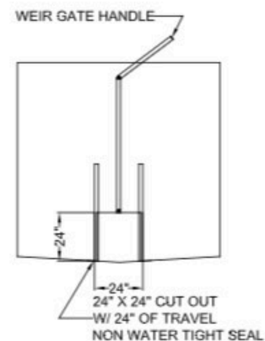
DETAIL A WEIR WALL DETAIL
