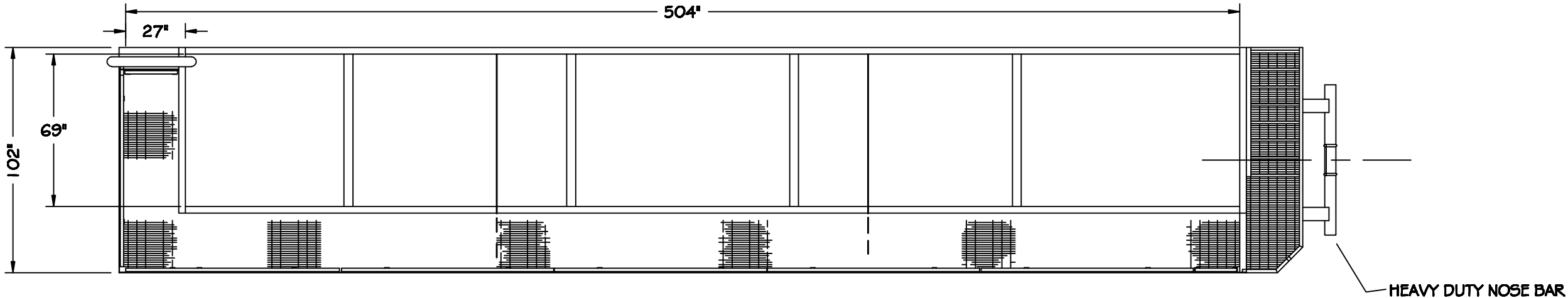
TOP VIEW.
