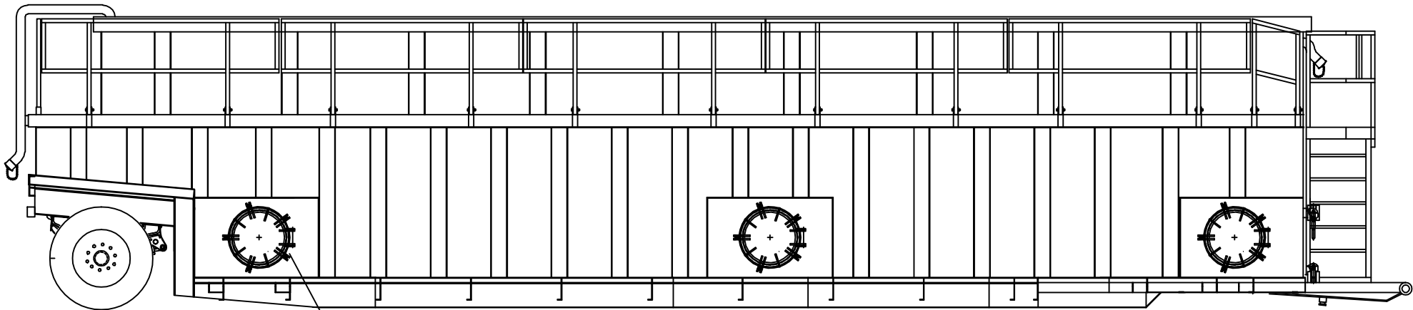
DRIVER'S SIDE ELEVATION VIEW.
